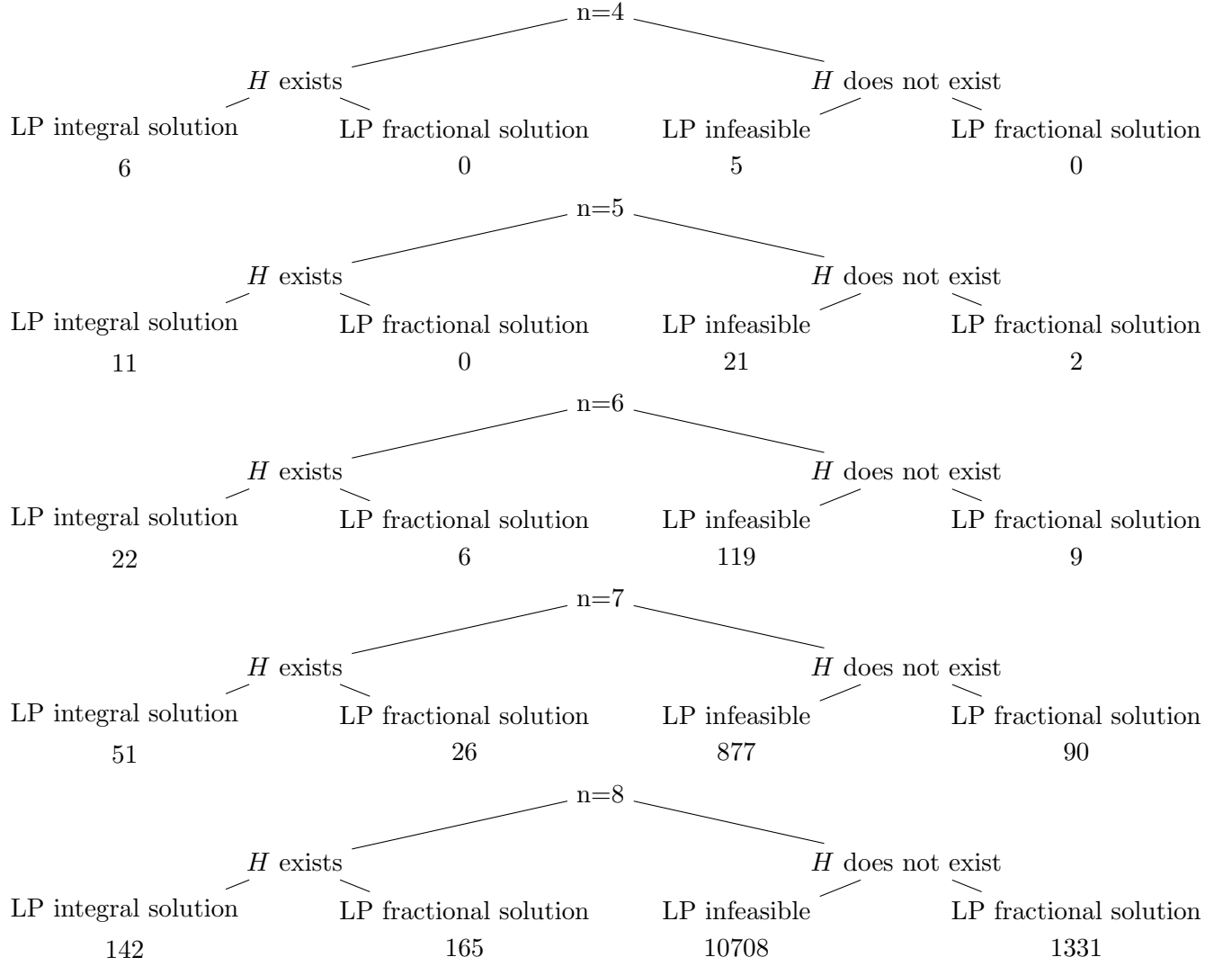
Figure 6: LP outcomes for different values of n on the linear program with max objective function and single triangular decomposition with recursion for tie-breaking.
