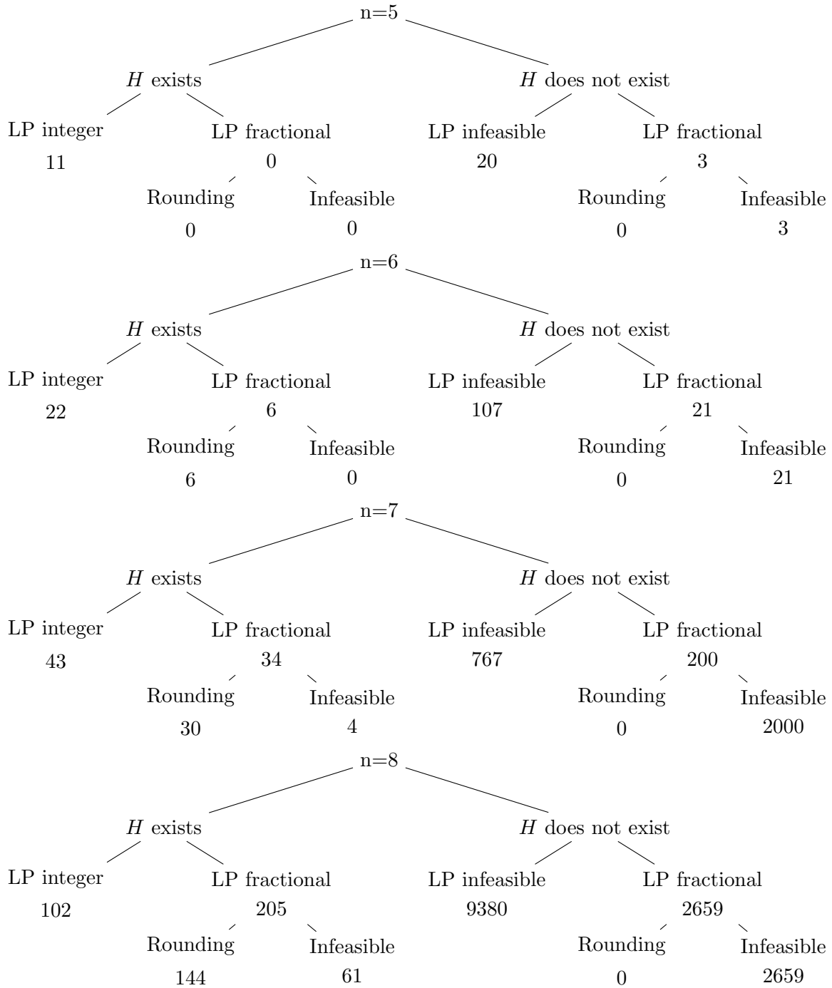
Figure 7: LP outcomes for different values of n on the linear program with max objective function and using rounding for fractional solutions.
