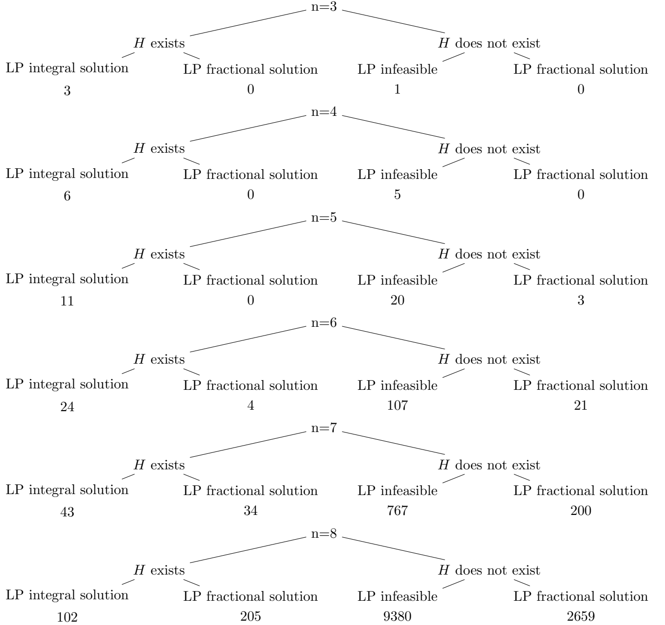
Figure 3: LP outcomes for different values of n on the linear program with max objective function.
