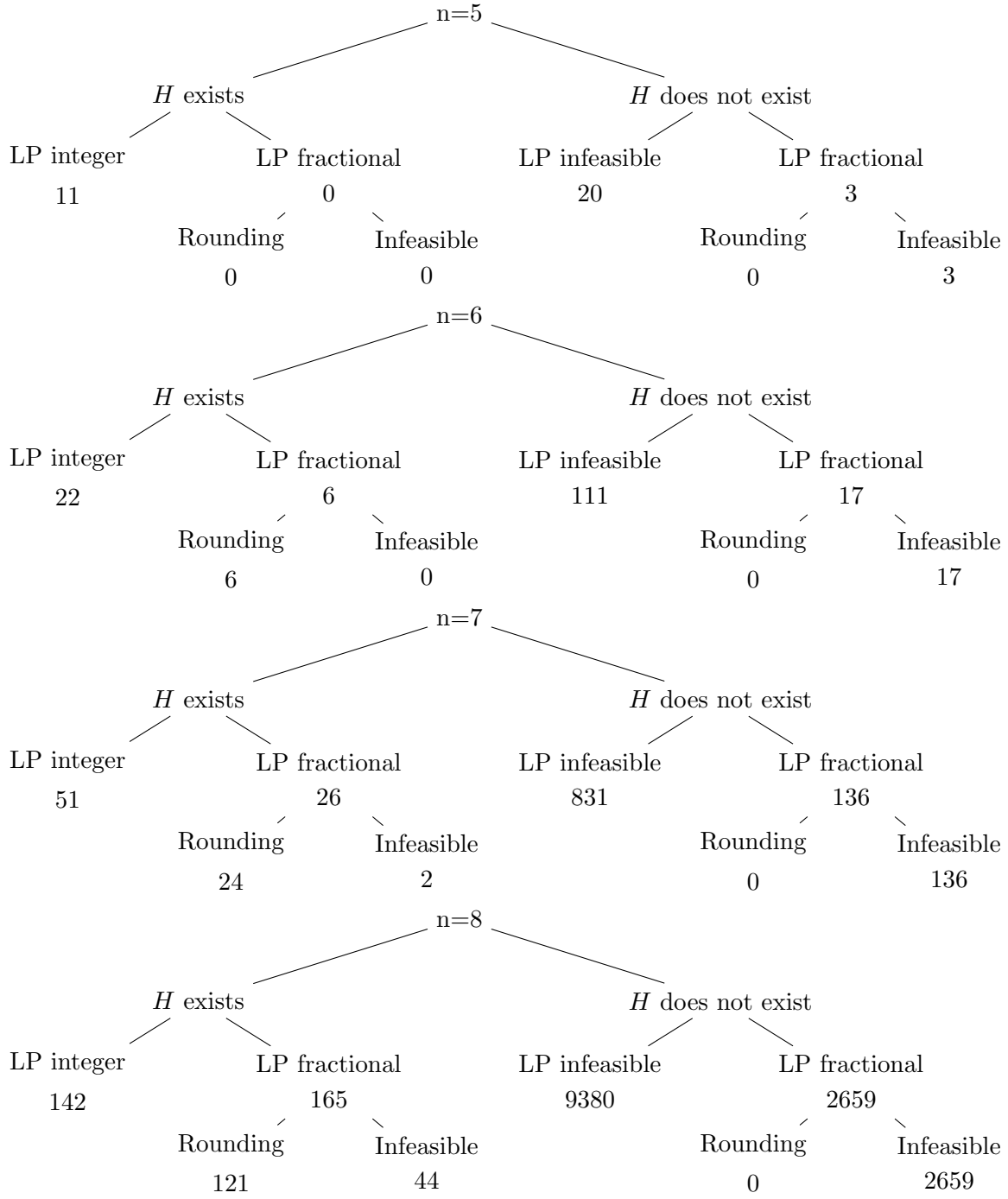
Figure 8: LP outcomes for different values of n on the linear program with max objective function, single triangular decomposition and using rounding for fractional solutions.
