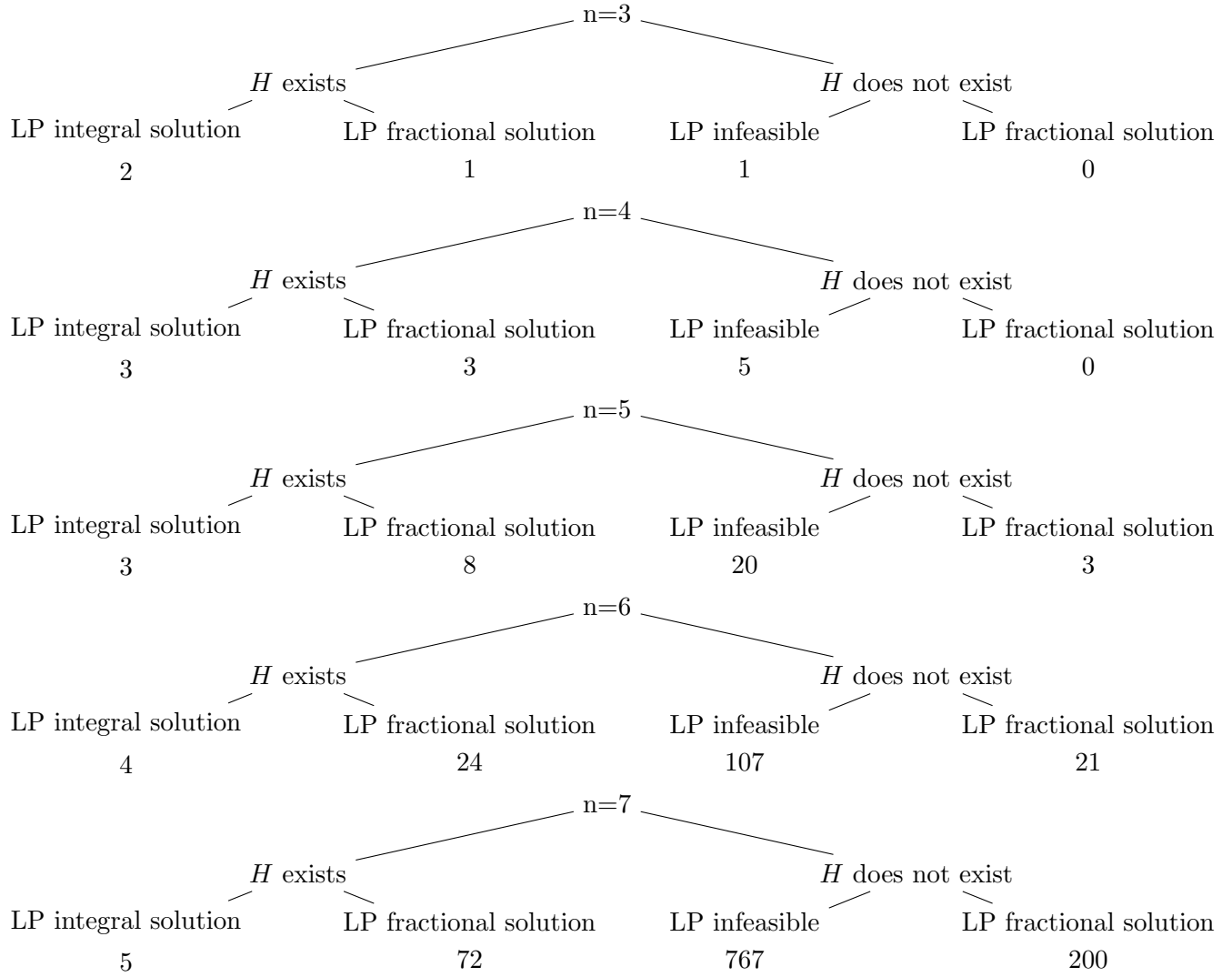
Figure 4: LP outcomes for different values of n on the linear program with min objective function.
