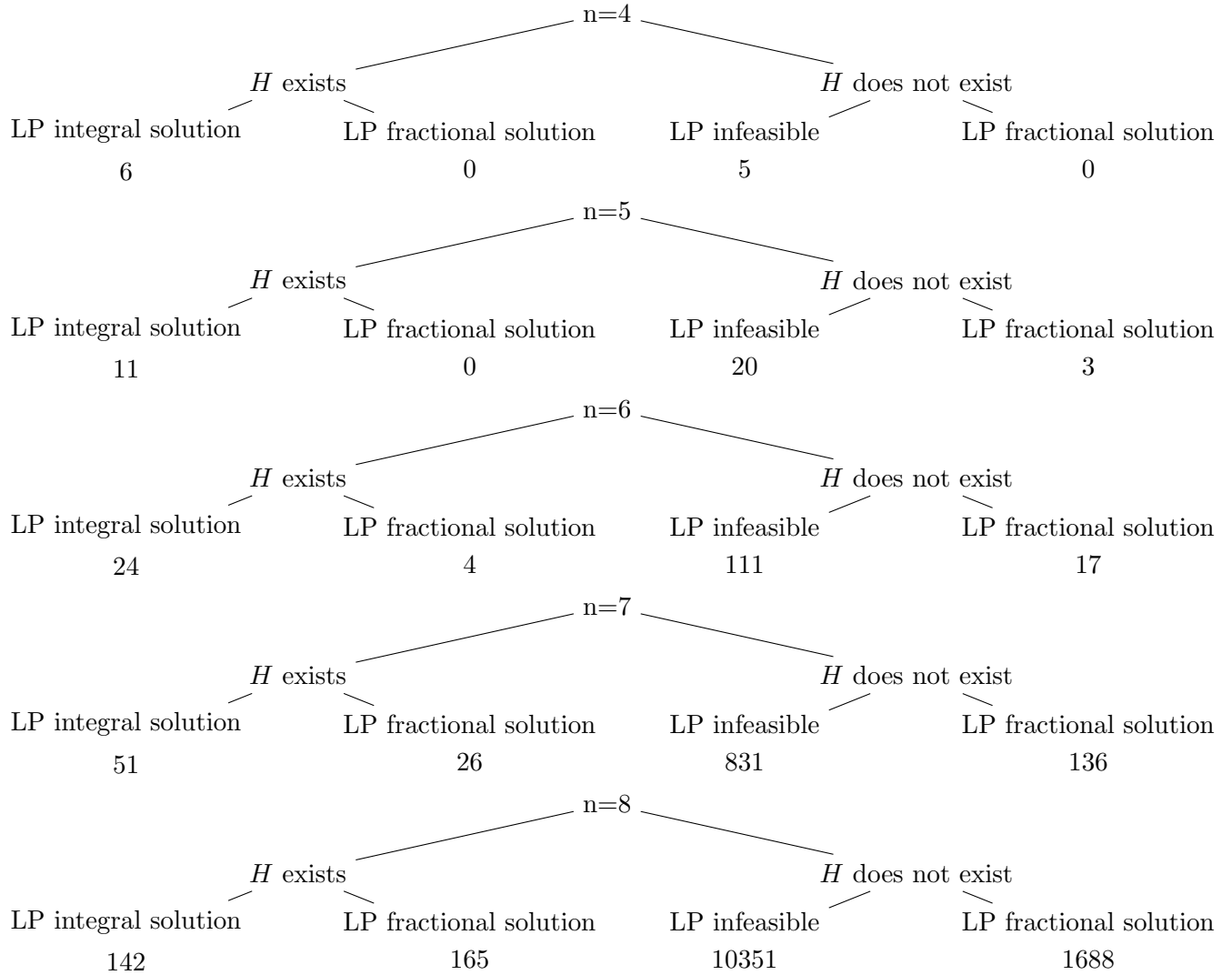
Figure 5: LP outcomes for different values of n on the linear program with max objective function and single triangular decomposition.
