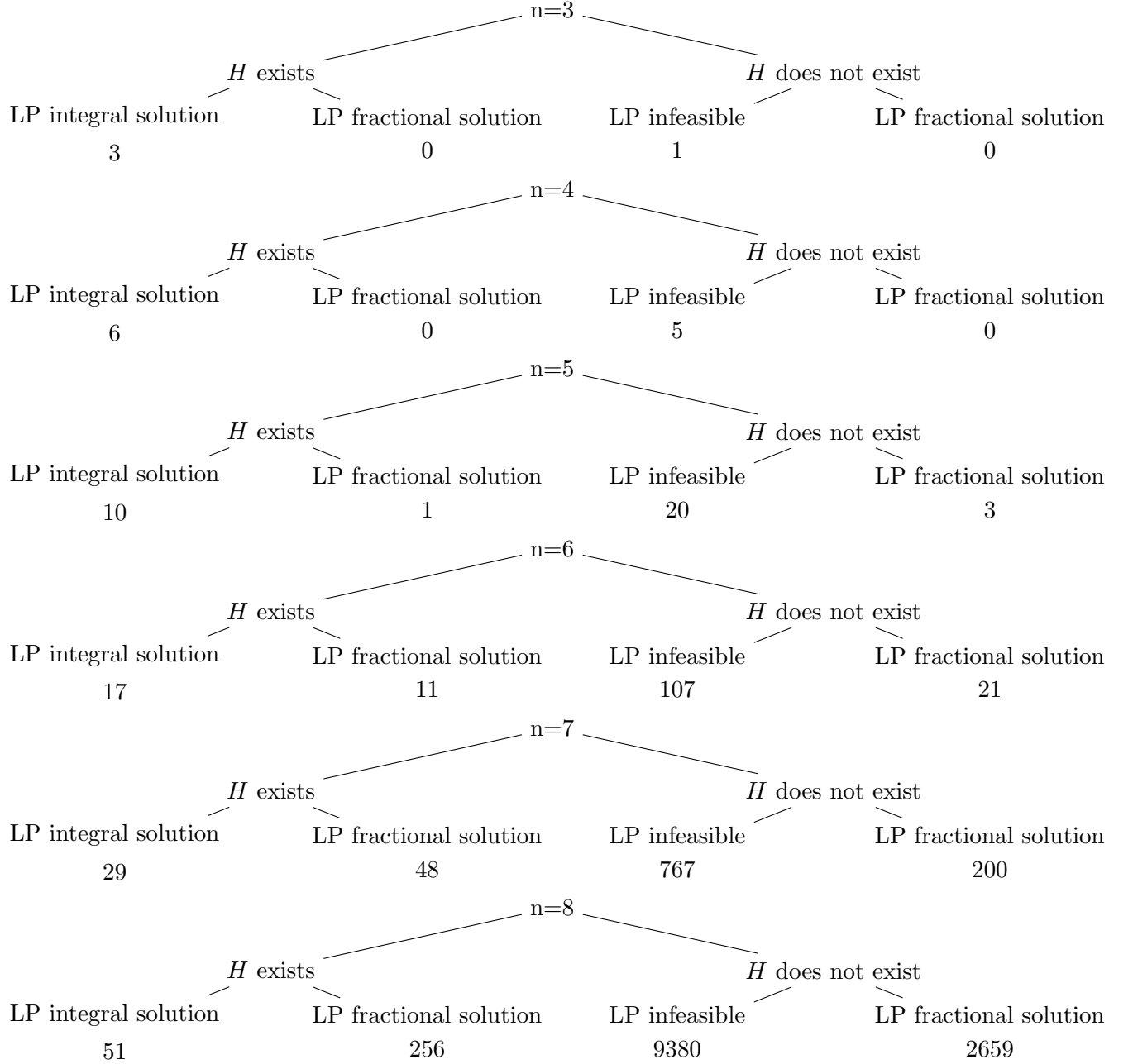
Figure 2: LP outcomes for different values of n on base linear program.
